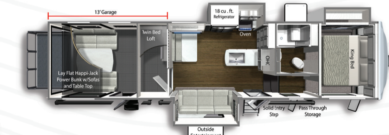
VOLTAGE 3675 Ext. Length: 39' 0" Weight: 14,020 lbs. Sleeps: 6-8 Hitch: 2,957 lbs. Height: 13' 3"
