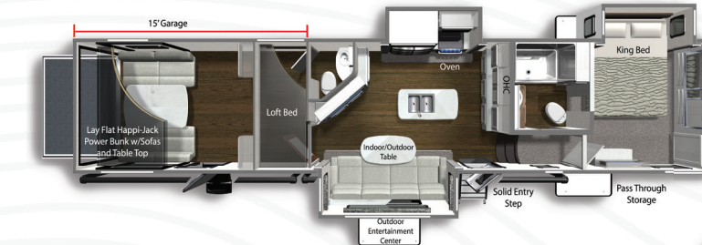
VOLTAGE 4135 Ext. Length: 44' 4" Weight: 15,269 lbs. Sleeps: 6-8 Hitch: 3,804 lbs. Height: 13' 3"
