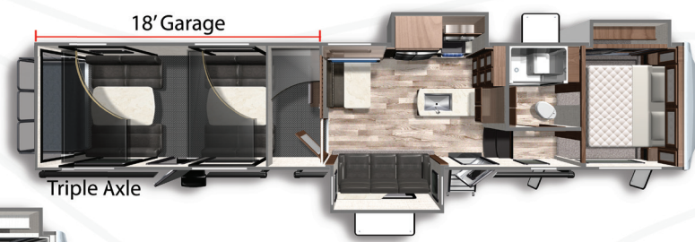
VOLTAGE 4145 Length: 44' 2" Weight: 15,545 lbs. Sleeps: 6-8 Hitch: 3,472 lbs. Height: 13' 3"
