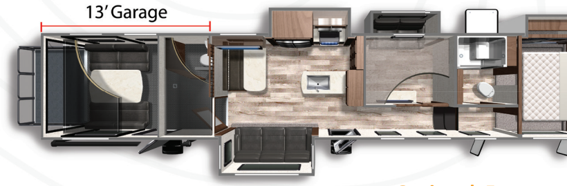
TRITON 4191 Ext. Length: 45' 1" Weight: 14,667 lbs. Sleeps: 4-6 Hitch: 3,657 lbs. Height: 13' 3"
